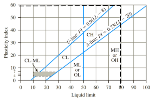
Figure 3. Plasticity Diagram (ASTM, Casagrande)
