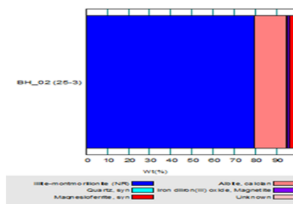
Figure 14. Test XRD mineral content of original soil sample
