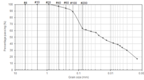
Figure 2. Gradation of original soil
