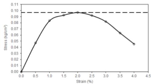
Figure 8. Stress strain from Unconfined Compression Strength test
