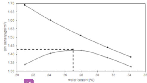
Figure 5. Maximum dry density v. Optimum water content
