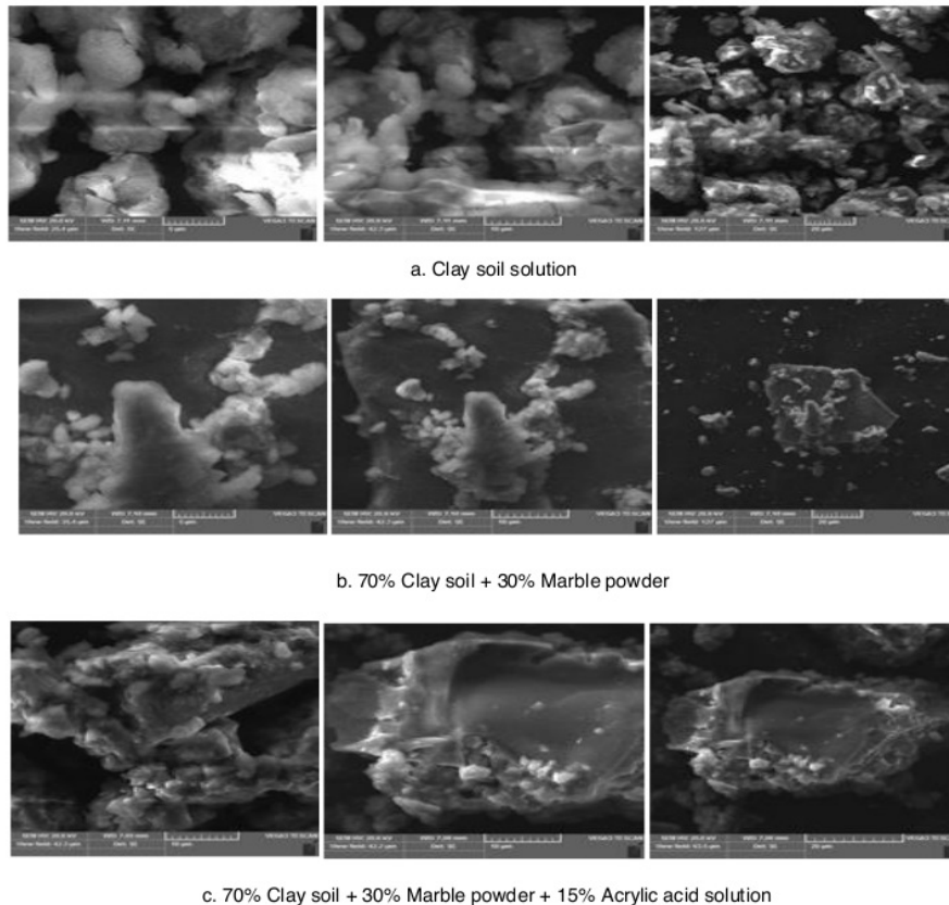
Figure 15. The result of SEM on mixture of clay soil, marble powder, and acrylic acid solution
