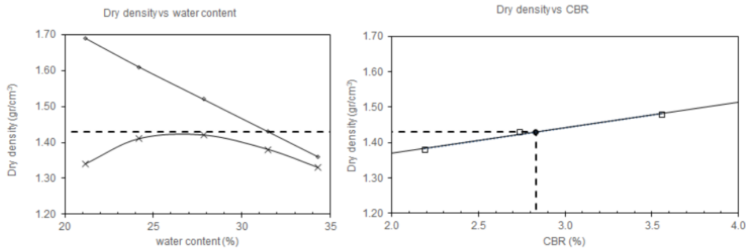
Figure 7. Determination of CBR design
