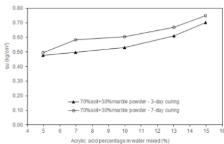
Figure 12. UCS values with 3 and 7-day curing.
